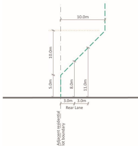
Figure 1 to Schedule 44 – Interface to residential properties in NRZ or GRZ
