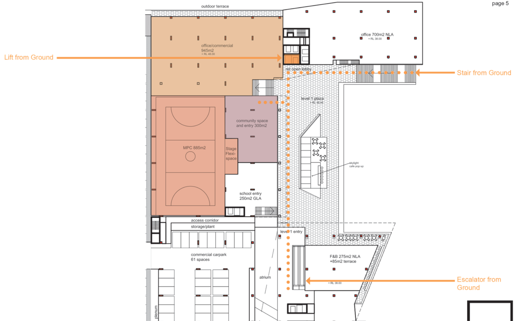
Level 1 Plan - Community Areas 1:400 @ A3
