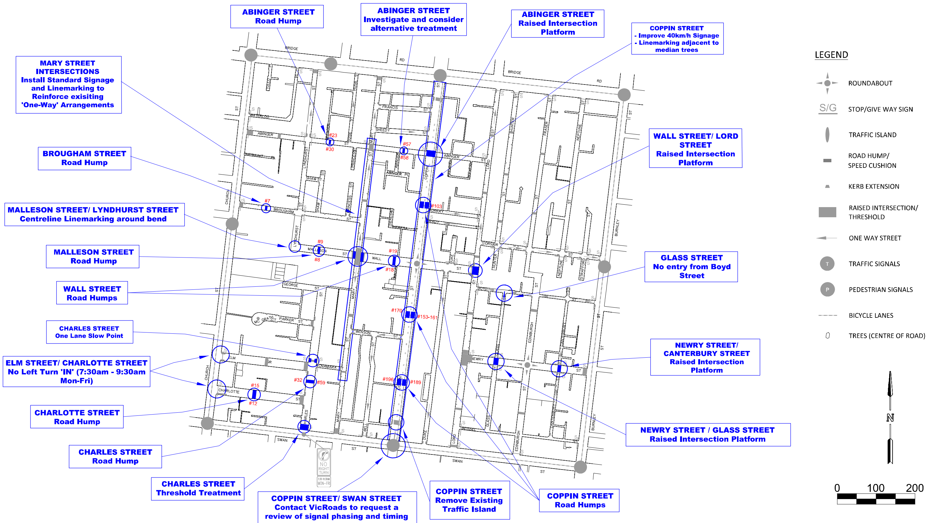
FIGURE 17: RECOMMENDED TRAFFIC MANAGEMENT PLAN
