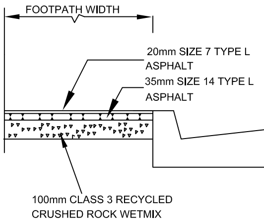
RESIDENTIAL ASPHALT FOOTPATH (RAF)
