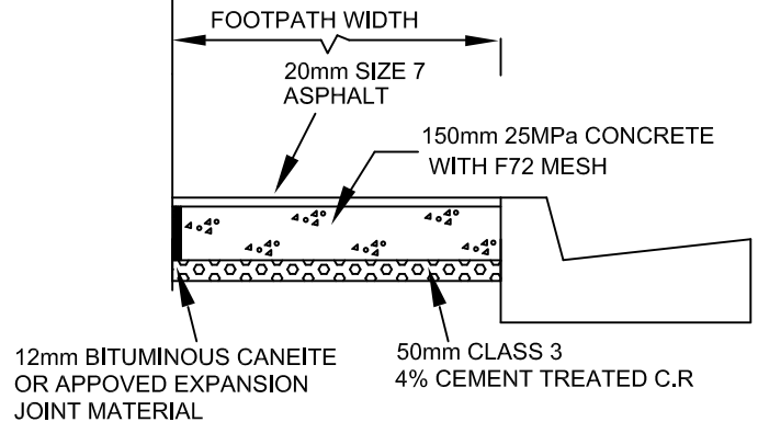
INDUSTRIAL CONCRETE FOOTPATH WITH ASPHALT SURFACE (ICAF)
