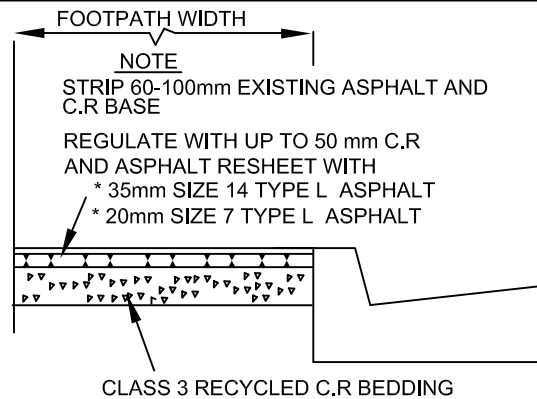
RESIDENTIAL FOOTPATH STRIP AND RESHEET
