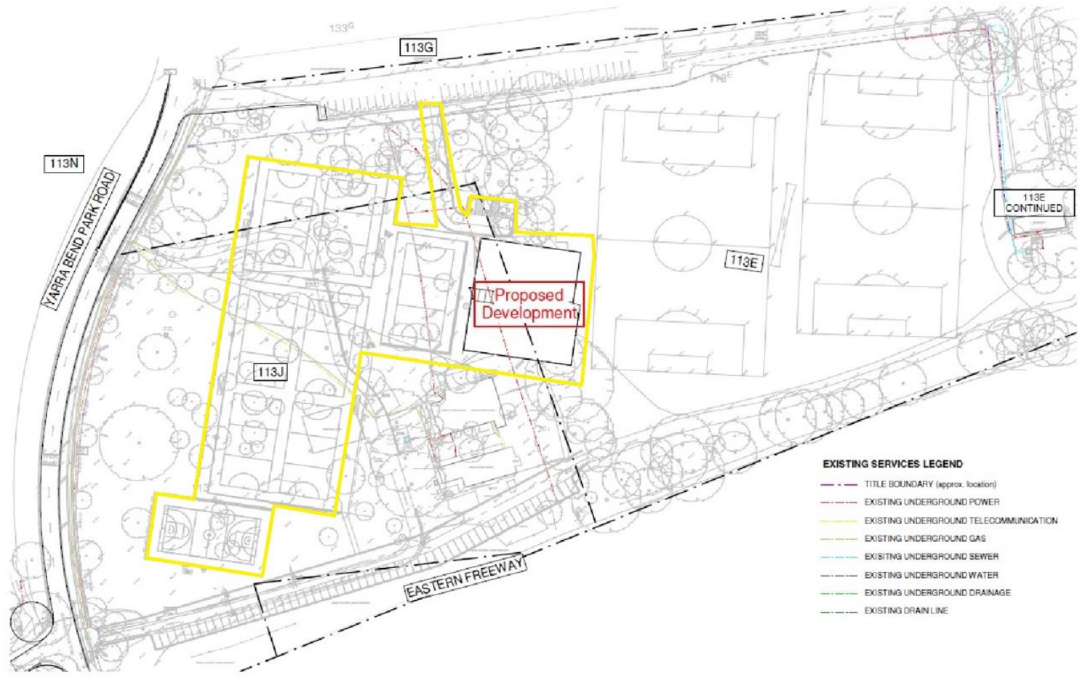
2 Proposed Site Plan 1 : 750
